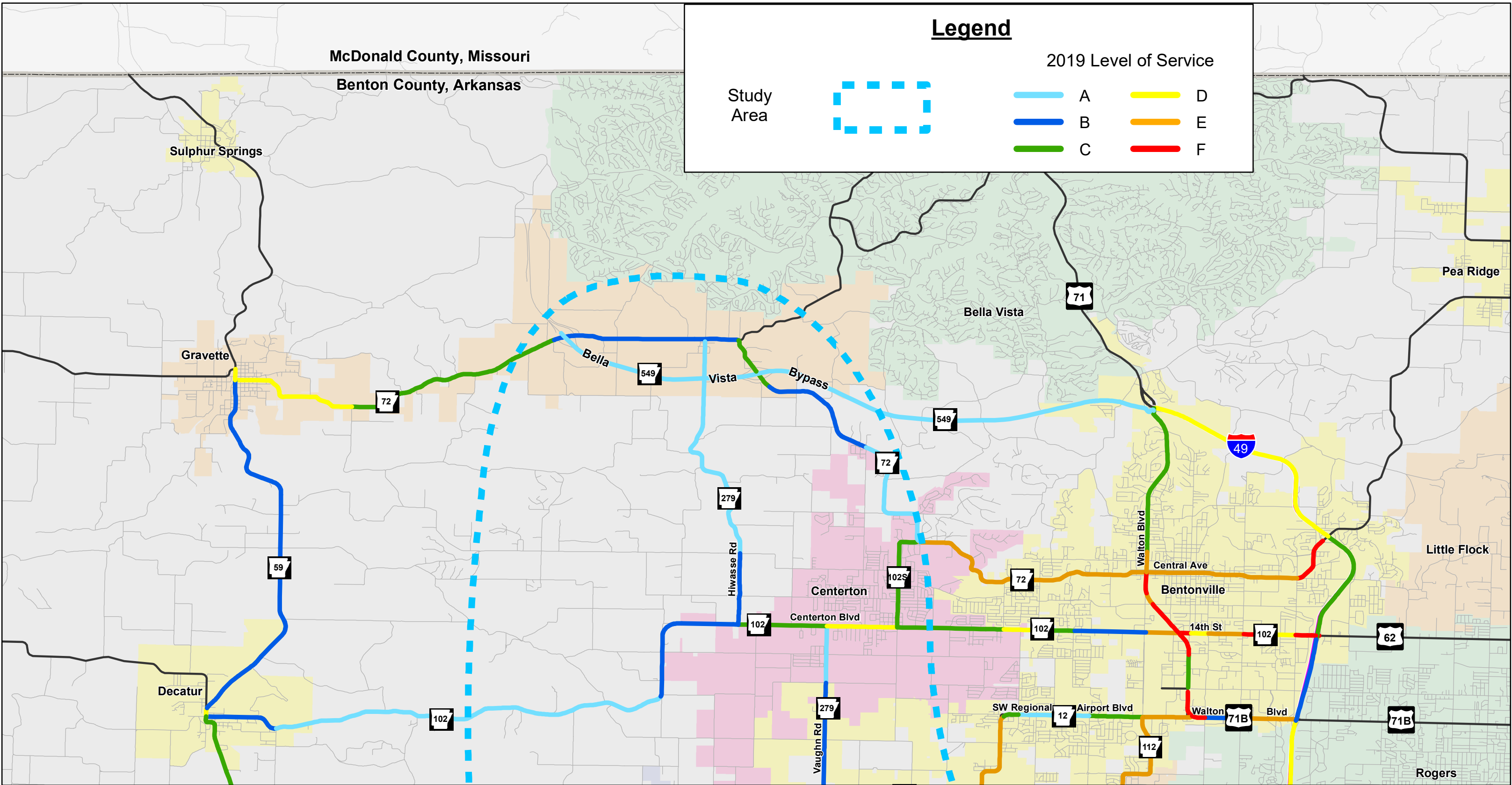
Western North-South Connector 2019 Existing w/ Bella Vista Bypass Level of Service Northern Study Area Map
